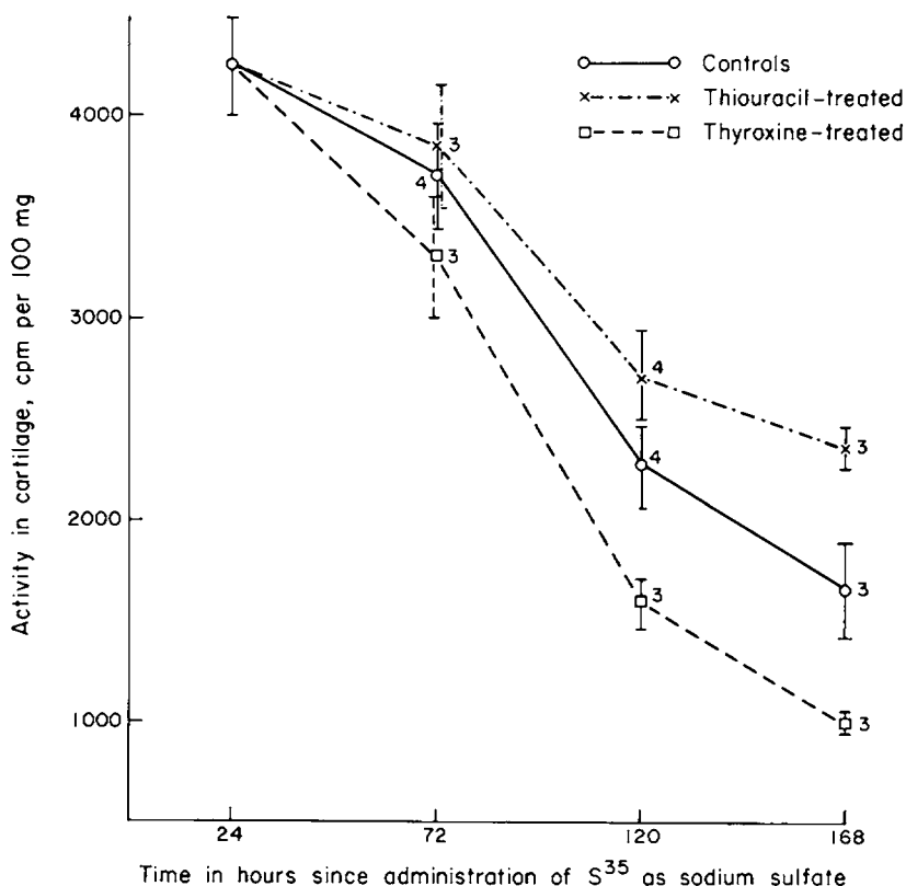
FIGURE 8 Effect of thyroxine and thiouracil on the disappearance of S^{35} from the cartilage of the knee-joints of suckling rats. S^{35} -sulfate was injected intraperitoneally on the 7th day of life. Into some of the rats 4 mg of thiouracil was then injected daily, intraperitoneally, starting with the 8th day of life. Other animals received 200 \gamma of thyroxine intraperitoneally on the 8th day of life and subsequently 100 \gamma doses on the 10th and 12th days of life. The number of animals used in obtaining a particular average value is shown by the numeral directly to the right of a plotted value. This figure originally appeared in J. Biol. Chem. , 1951, 189, 717.
