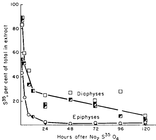
FIGURE 3 Recovery of S^{35} as inorganic sulfate from extracts of epiphyses and diaphyses removed from suckling rats at intervals of time following administration of Na_2 S^{35} O_4 . The extracts were prepared by the use of a 2.5N solution of NaOH. The inorganic sulfate was separated from other S^{35} -labeled materials by chromatography on columns of Dowex — 2 \times 10 . This figure originally appeared in J. Exp. Med. , 1957, 106 , 509.
